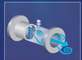
Vortex flowmeters
