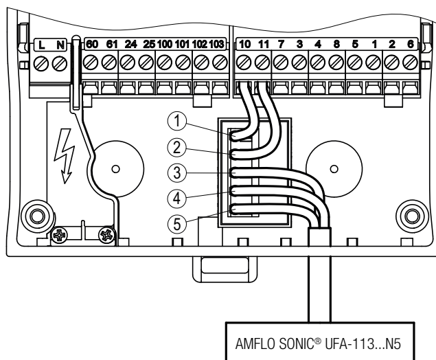
CALEC® ST / Namuradapter 5V / AMFLO® SONIC UFA-113...N5
