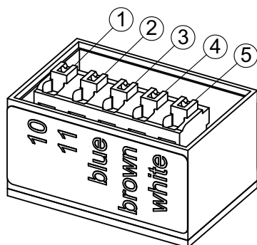
Namuradapter 5V: ID 80661
